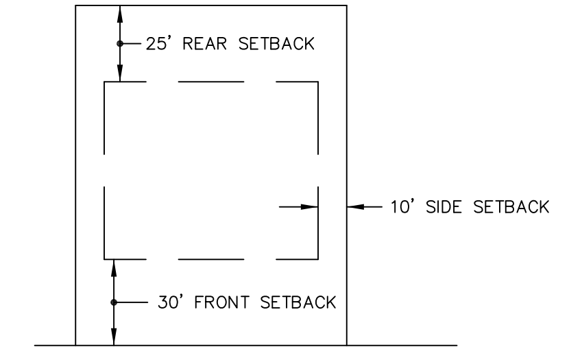
TYPICAL LOT DETAIL NOTE: 20.0' MINIMUM DISTANCE BETWEEN BUILDINGS
